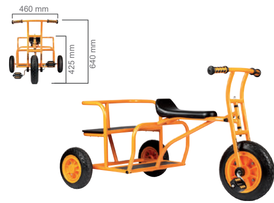
Pillion Taxi 64140 (L1130 W680 H640mm) 44.5x26.8x25.2inches The tricycle "Pillion Taxi" offers room for up to three children. One child can drive the sturdy vehicle and up to two kids can enjoy the ride while sitting on the back seat.
